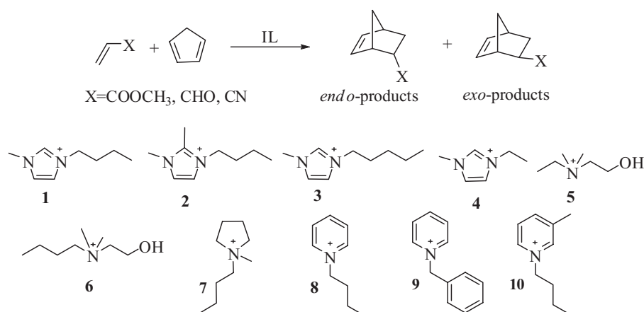
Scheme 1. Diels–Alder cycloadditions studied and ionic liquid cation structures employed; in all cases as the [\text{TF}_2\text{N}]^- salts
